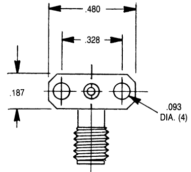
MOUNTING (b)
