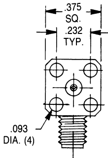
MOUNTING (a)
